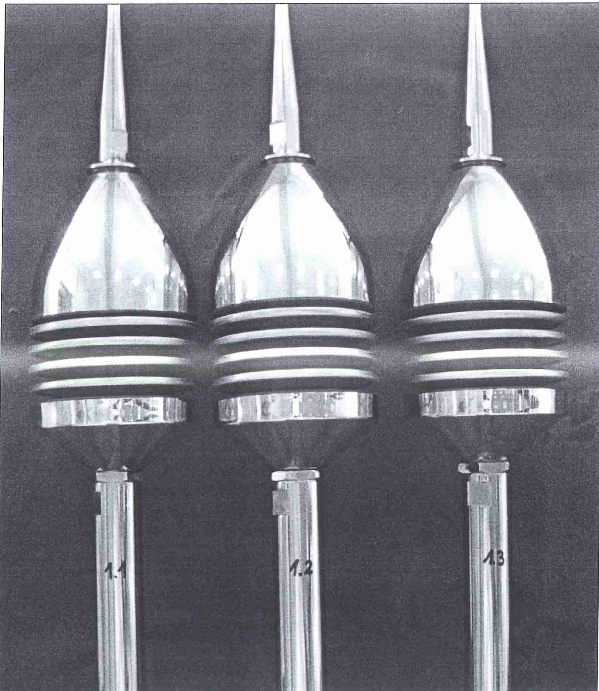
Figure 2: DUT after the impulse current test
